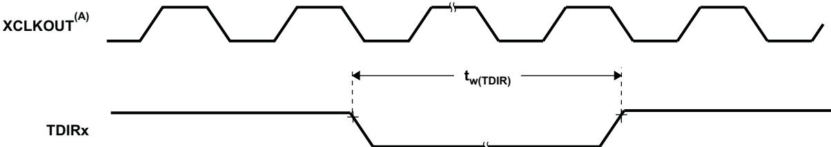
Figure 6-19. TDIRx Timing
