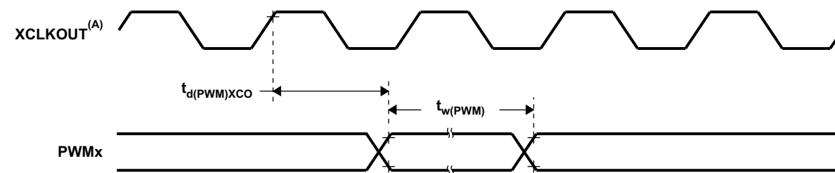
Figure 6-18. PWM Output Timing
